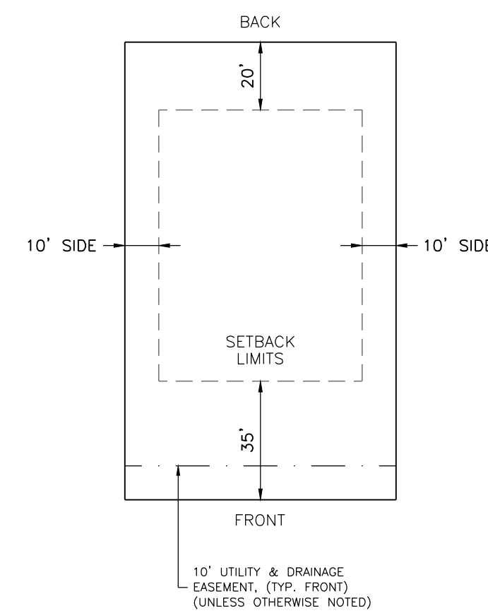
TYPICAL LOT DETAIL N.T.S.
